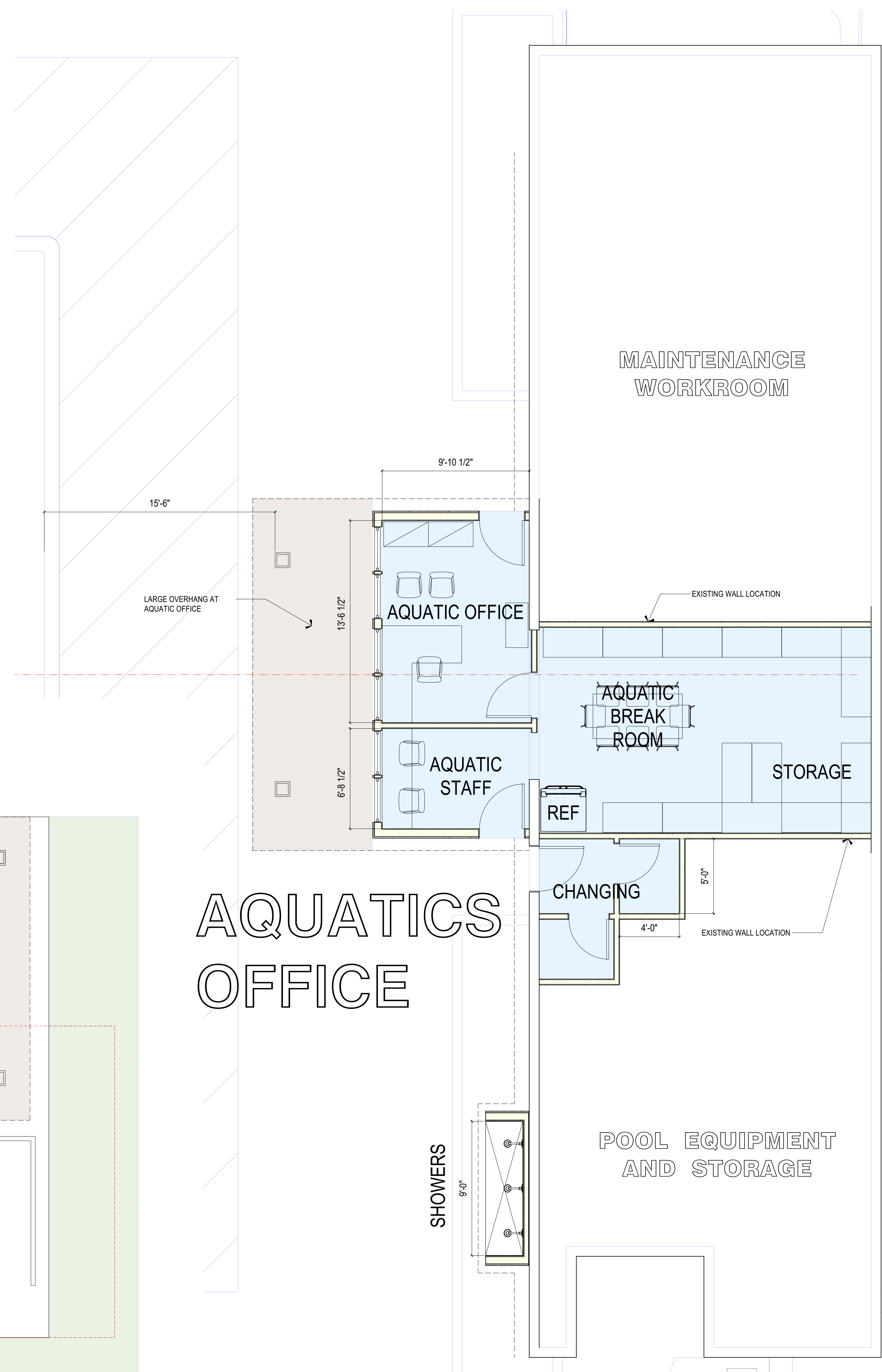
AQUATICS 2 Scale: 1/4" = 1'-0" A2.3
